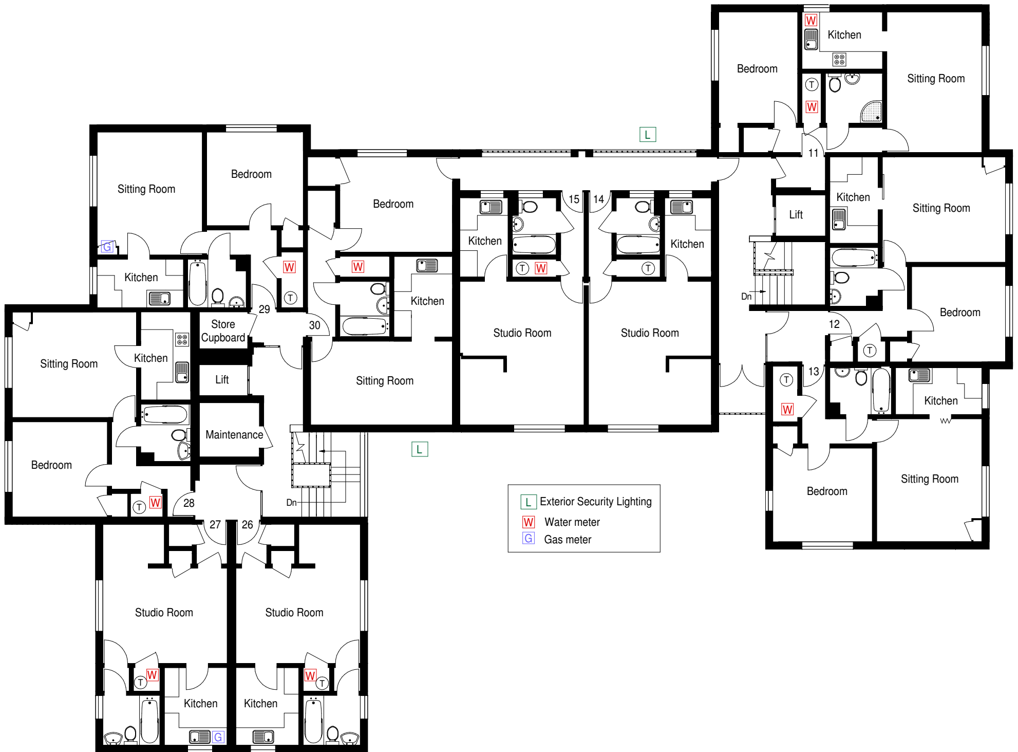
Second Floor
